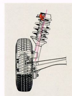
The offset springs reduce damper friction and road noise.
