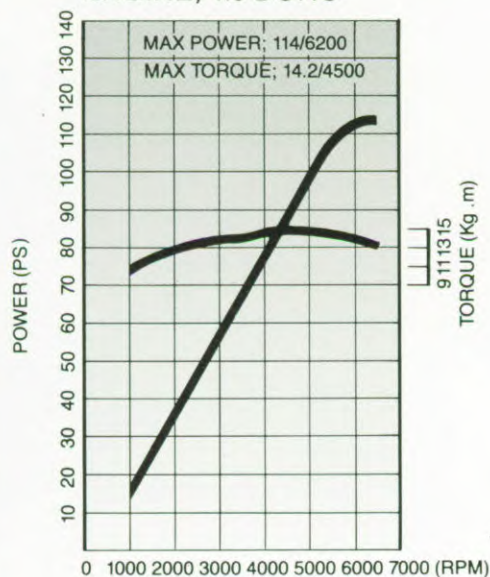
ENGINE; 1.6 DOHC
