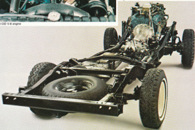
Rugged Wagoneer chassis
