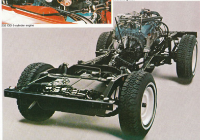
Suggested CJ chassis (V-8 engine optional)
