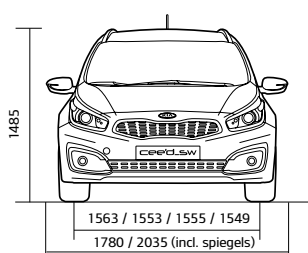
cee'd Sportswagon buitenafmetingen (mm)
