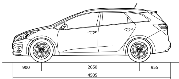
cee'd Sportswagon buitenafmetingen (mm)
