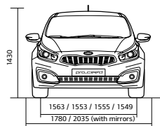
pro_cee'd 3-door exterior dimensions (mm)
