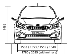
cee'd Sportswagon exterior dimensions (mm)
