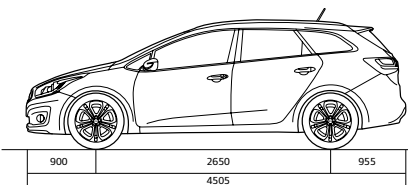
cee'd Sportswagon exterior dimensions (mm)
