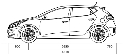
cee'd 5-door exterior dimensions (mm)
