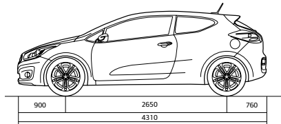
pro_cee'd 3-door exterior dimensions (mm)
