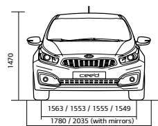
cee'd 5-door exterior dimensions (mm)
