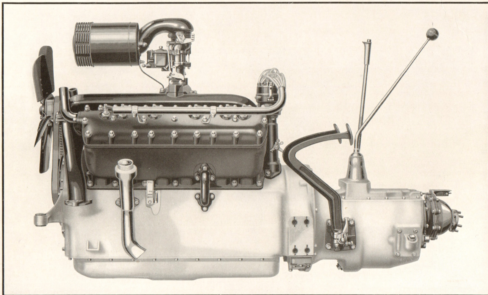
THE LINCOLN V-12 CYLINDER 125 HORSEPOWER ENGINE
