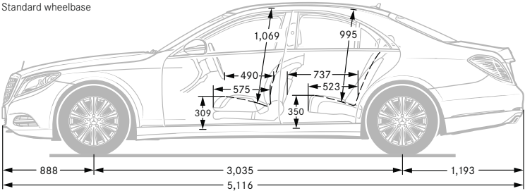
Standard wheelbase
