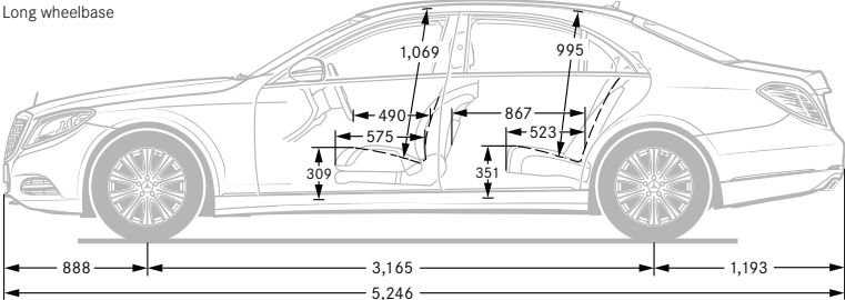
Long wheelbase
