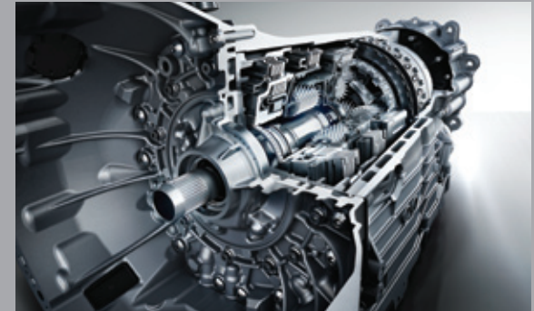
7G-TRONIC PLUS
