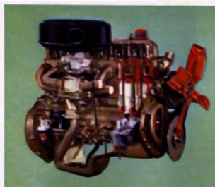
Responsive Skybolt Six —112 H.P.—spirited performer (154 ft. lbs. of torque), remarkably economical. New piston design and improved carburetion give even better performance. Meets every demand of today's high-speed highway driving at minimum cost.
