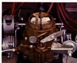
Two New Carburetors. All V8's from Studebaker Corporation now have an improved 2-barrel carburetor as standard equipment. They provide better economy, surer starting and are designed to reduce icing and stalling. A special 4-barrel model is optional for extra power.
