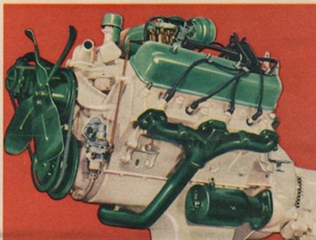
The new Commander V-8 "Pace-setter" engine
