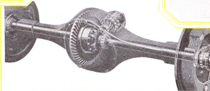
A "phantom" view of the special heavy duty rear axle—note the heavy box section housing and large shafts.
