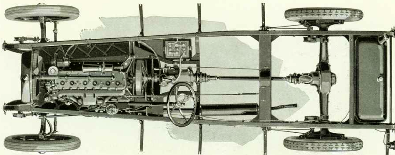
The BIG-SIX Chassis
