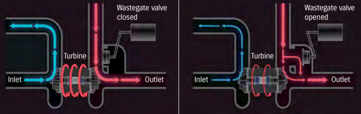
Closed for normal driving, it helps apply higher boost pressure to achieve excellent torque response. Opened for cruising, it prevents overpressure and suppresses fuel consumption.
