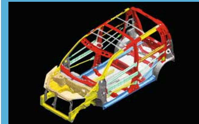
Energy absorbing body structure for safer drives
