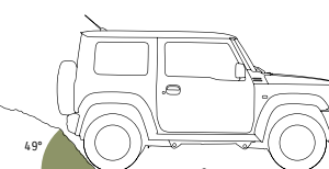
Departure angle
