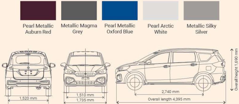
The drawings shown are general specifications of the vehicle.
