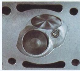
2. The triple hemisphere swirl action combustion chambers achieve optimum mixture distribution and smooth combustion. The result: unique development of power, favourable exhaust ratios and economic consumption.
