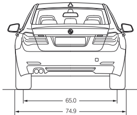
All dimensions in the technical drawings are given in inches. Figures in ( ) refer to the 750i (short-wheelbase version).
