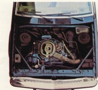
2.8 Litre V6 Engine. A totally new engine designed for the 1980 Chevy Citation. Features compact design with aluminum inlet manifold, water pump housing, engine front cover and carburetor. Strong cast-iron cylinder block and heads, yet is relatively light in weight.
