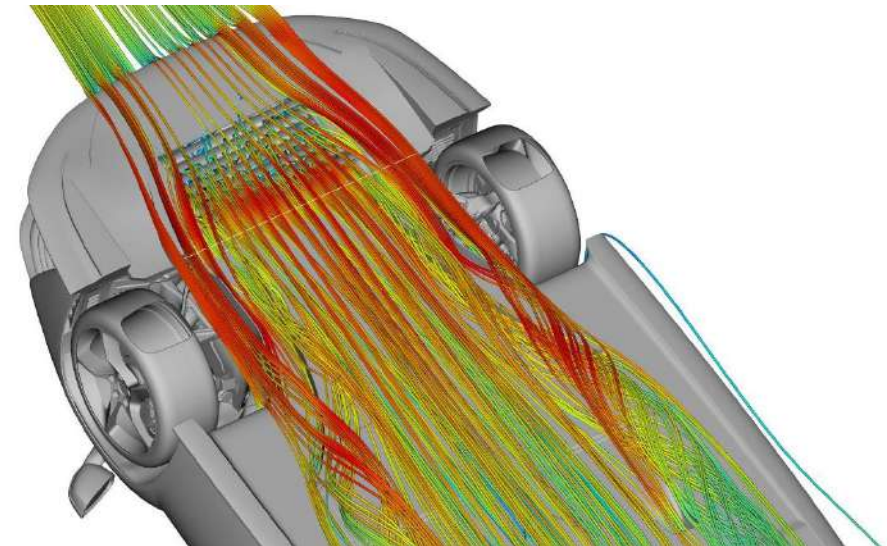
Fig. 19 - Aerodynamic sealing effect of the vortex generator on the front underbody
