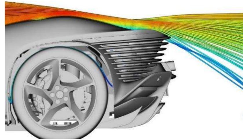
Fig. 20 - Pressure distribution on the rear bodywork and the flow to the spoiler
