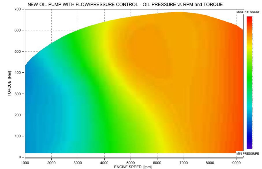
Fig. 8 - Oil-revs/torque pressure regulation
