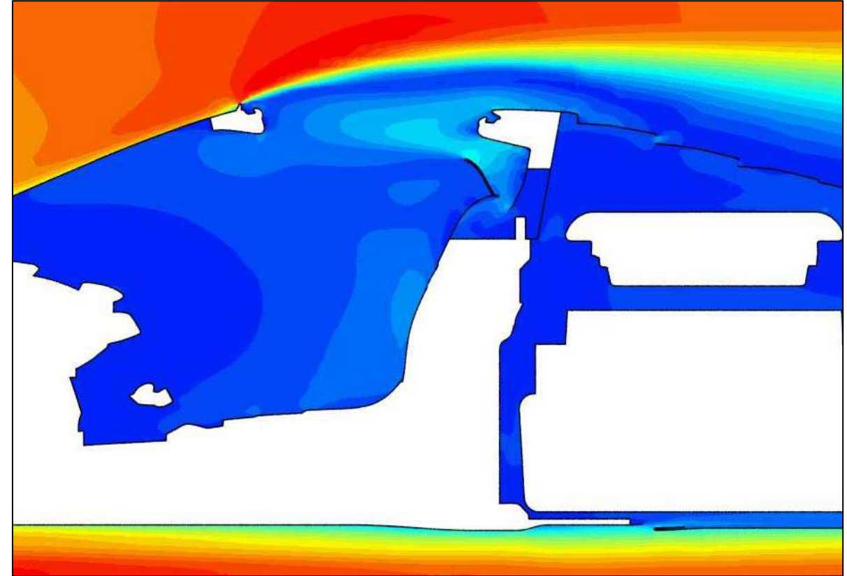
Fig. 24 - Interaction between the windshield nolder and the cabin: the turbulent wake is deflected upward to prevent it re-entering the rear area of the cabin
