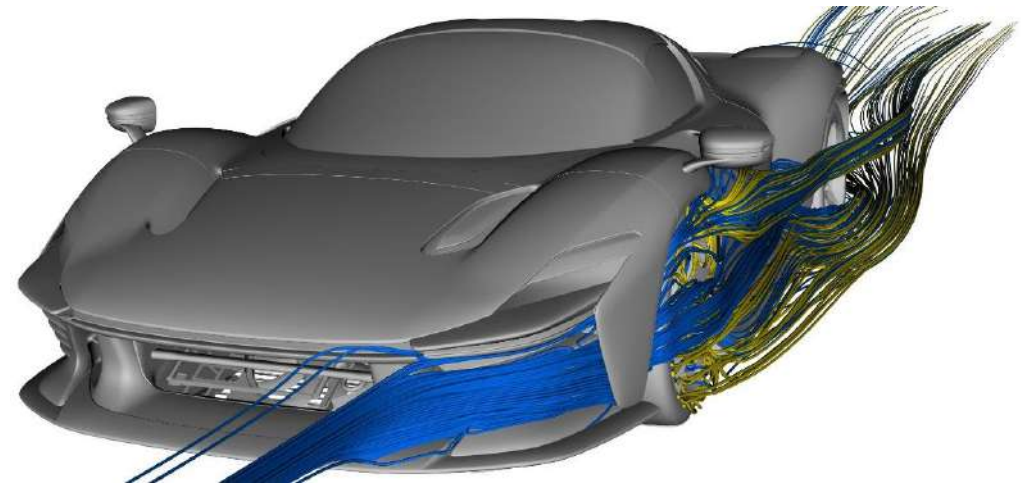
Fig. 16 - Synergy between vented side bumper and wheel to manage the flow along the flanks: the flow continues to hug the car's flanks, reducing the size of the car's wake
