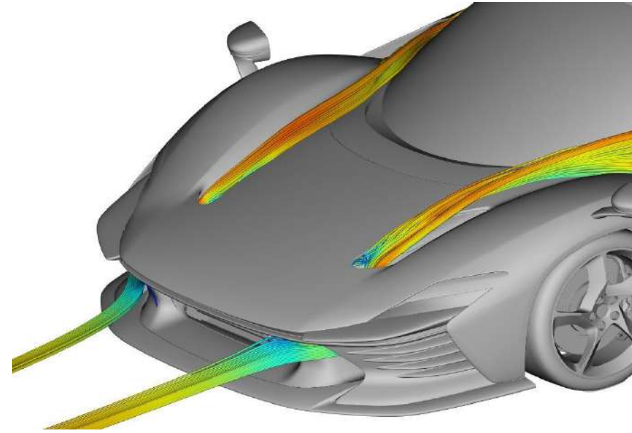
Fig. 15 - Blowing along side of bonnet: flow lines created by ducts
