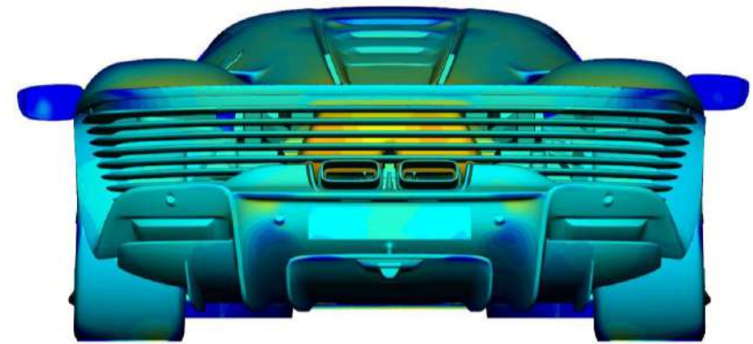
Fig. 23 - Double central diffuser: the central bridge is flanked by a more external diffuser volume that enhances its efficiency
