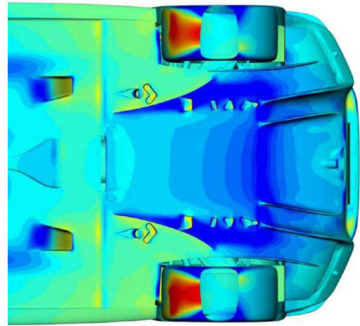
Fig. 22 - Pressure distribution on rear diffuser: space freed up between the wheels is used to expand the flow from the underbody in the diffuser
