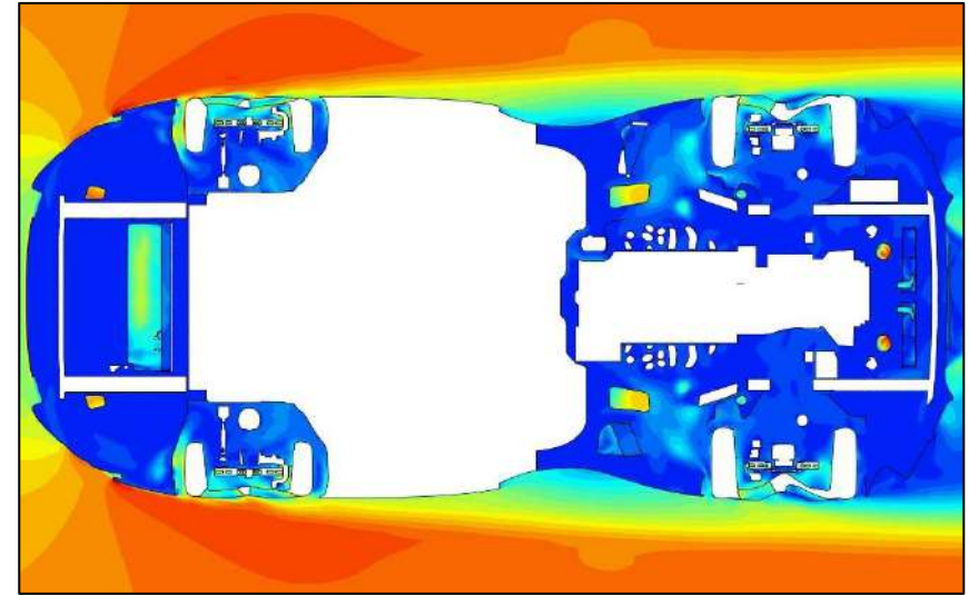
Fig. 17 - Synergy between the vented side bumpers and wheel to manage the flow along the flanks: the flow hugs the flanks, reducing the car's wake
