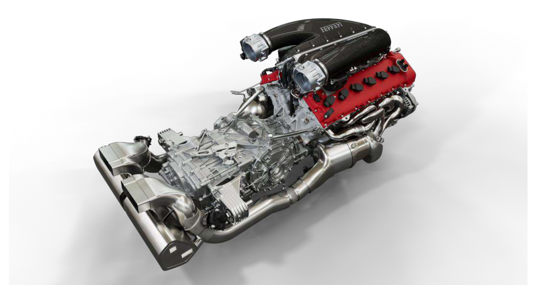
Fig. 10 - Twin-tailpipe exhaust system
