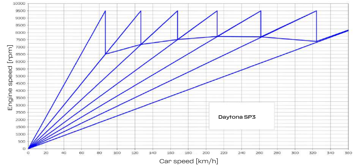
Fig. 11 - Gear ratios
