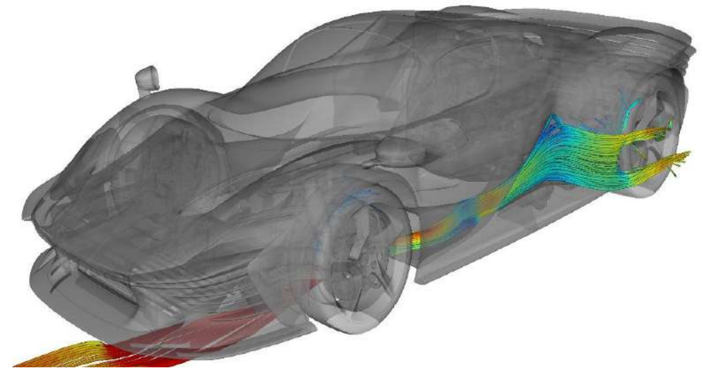
Fig. 18 - Close-up of the evacuation of the overpressure in the wheel well in the duct under the flank
