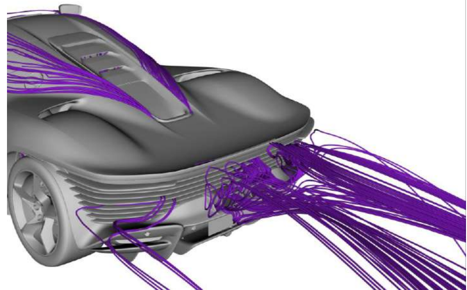
Fig. 14 - Interaction between the apertures on the sides of the backbone and the rear grille to guarantee the required cooling flow to the engine compartment
