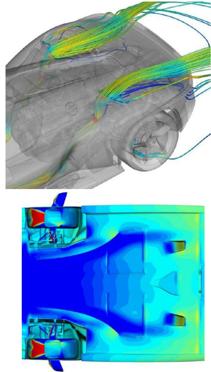
Fig. 21 - Suction generated on the underbody by the shape of the intakes: the front ramp is similar in shape to a diffuser
