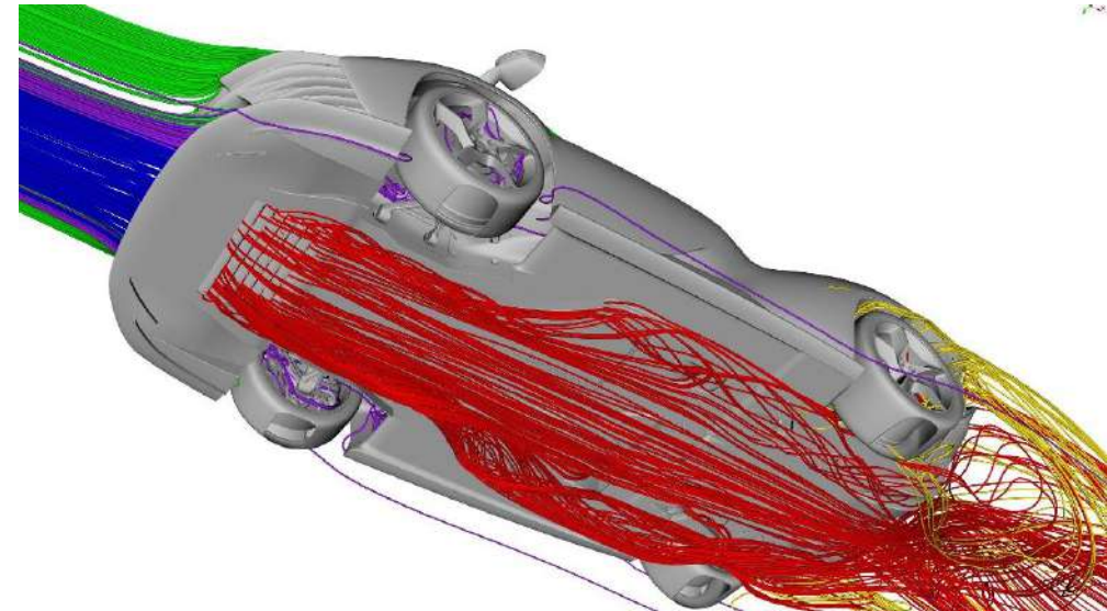
Fig. 12 – Car cooling flows and heat evacuation: blue/red engine and air con water, green/yellow engine-gearbox-clutch, purple brakes
