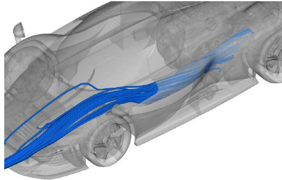
Fig. 13 - Side radiator intakes integrated into the doors
