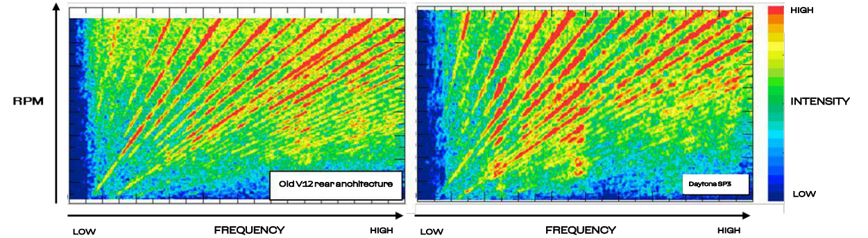
Fig. 9 - The sound pressure spectrum in the cabin as revs rise. The unusual intake layout lends the classic harmonics of the Ferrari V12 a greater intensity in mid frequencies, yielding a signature timbre that only adds to the car's sporty allure
