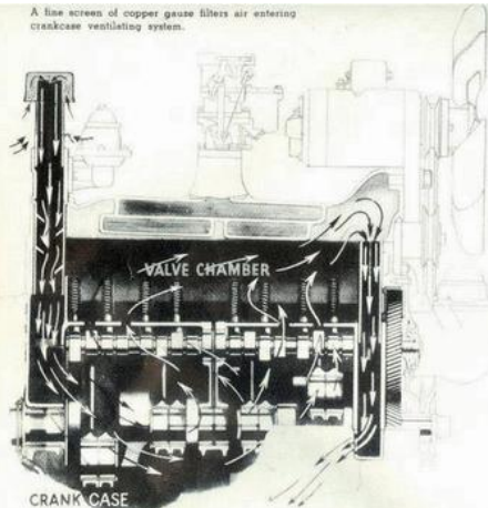
A line screen of copper gauze filters air entering crankcase ventilating system.
