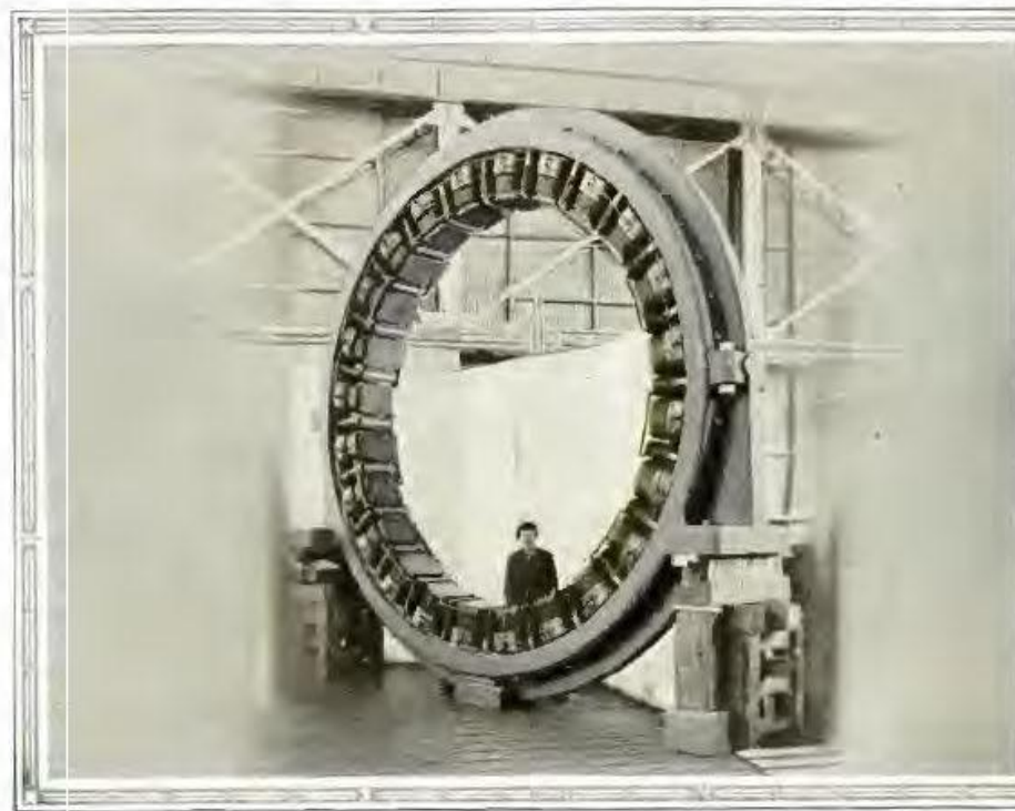
THE NEW GENERATOR nearing completion. 2500 K. W., 25% overload, diameter of frame 20 feet. The largest 240 volt dynamo ever built
