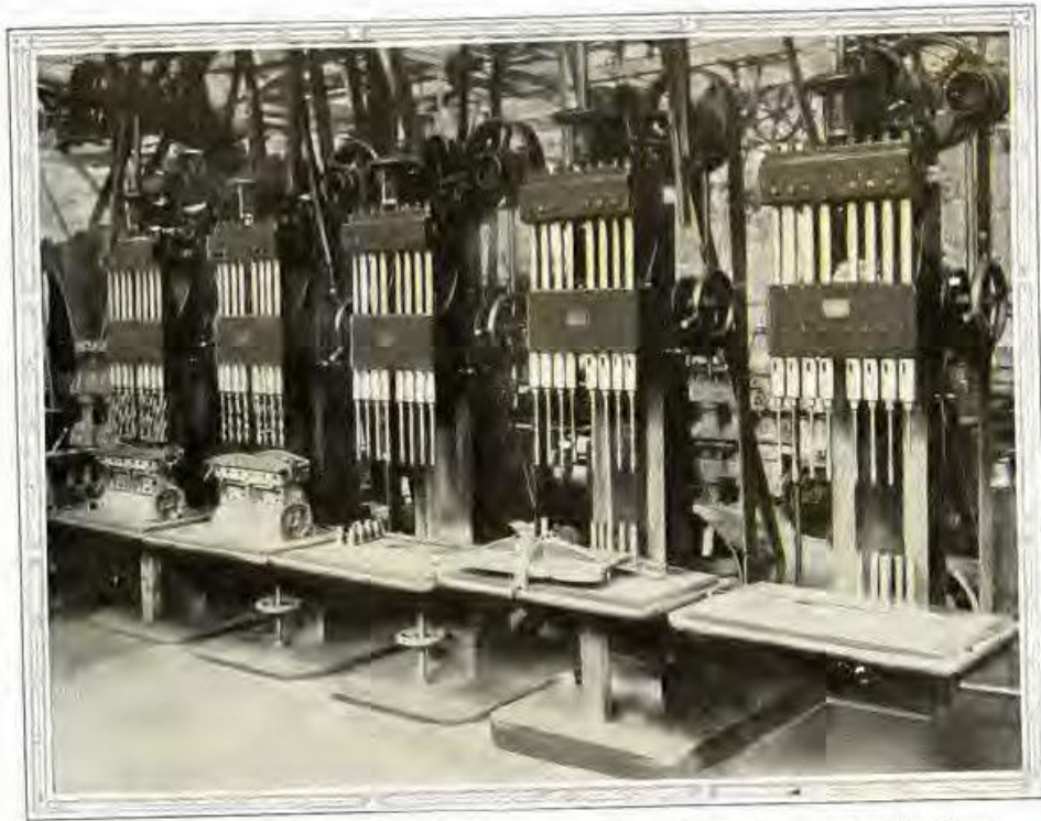
A BATTERY OF DRILLS —Each bores eight holes simultaneously, obtaining both absolute precision and great economy in time and labor
