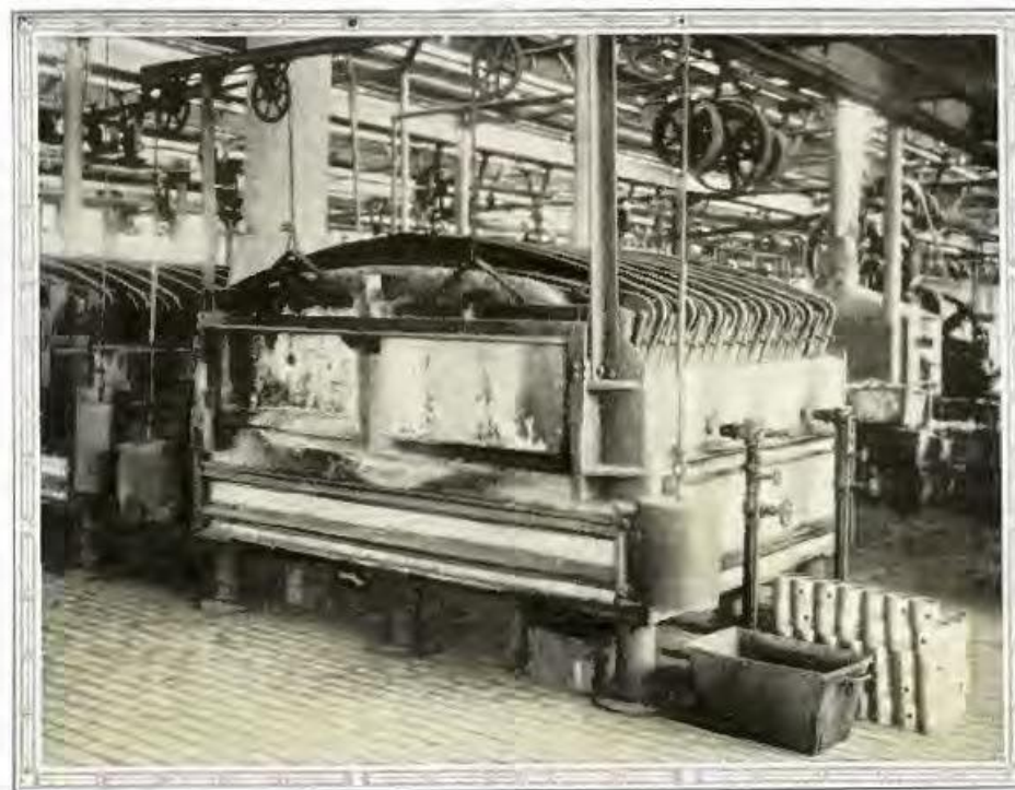
THE TYPE OF FURNACE used in the Heat Treating and Carbonizing Departments. Heated by two blazing jets of oil
