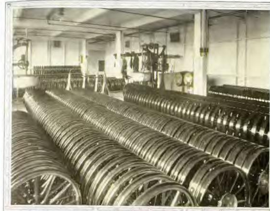
VARNISHING FORD WHEELS —Each machine varnishes two wheels per minute—1200 daily—and more perfectly than by hand
