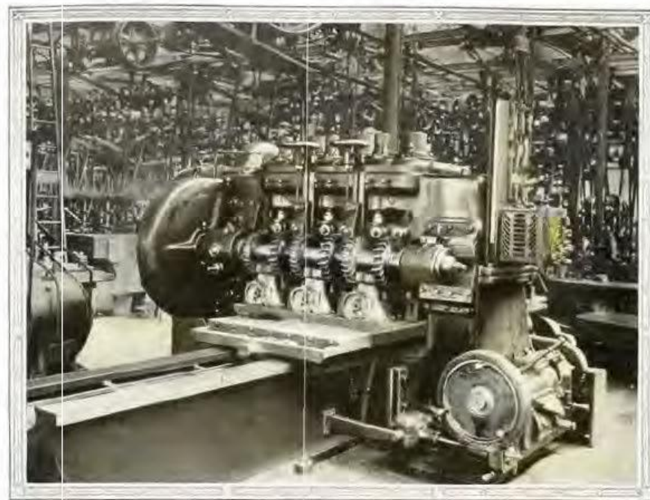
A MONSTER MILLING MACHINE , milling 12 cylinder castings at one operation. The massive cutters eat through the solid iron as if it were cheese
