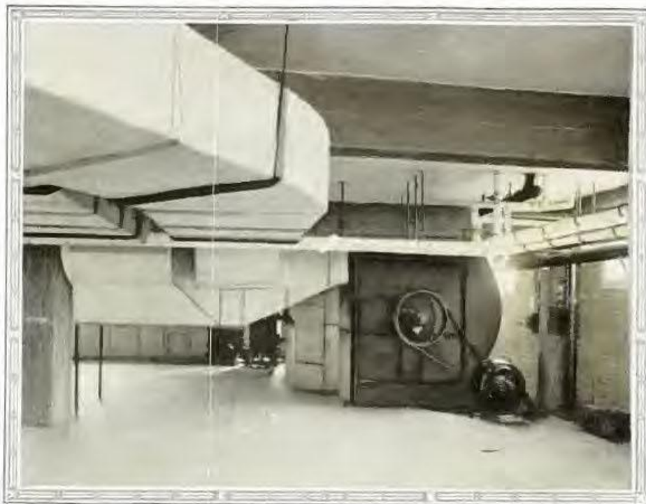
HUGE VENTILATING FAN —Two of these supply fresh air, purified through a water spray and heated to a uniform temperature, to each room
