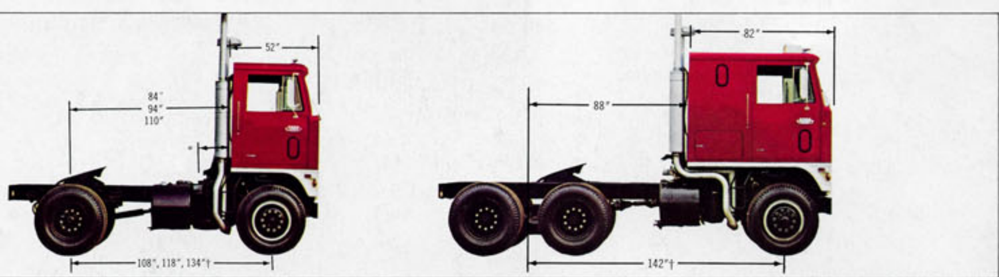
W-1000-D (52" BBC short cab shown). GCW: 65,000—80,000 lb. *Engines project from 1" to 14". †Other tractor wheelbases to order.
