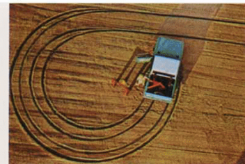
Turning . . . The Bronco turns in a 33.6-ft. diameter . . . less than any other comparable utility vehicle. This ability to turn in a small area comes in mighty handy going round obstacles.
