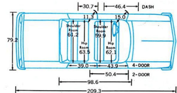
STATION WAGON DIMENSIONS*
