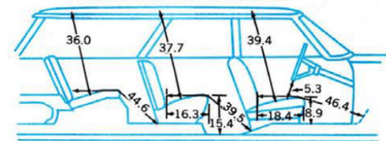
STATION WAGON DIMENSIONS*
