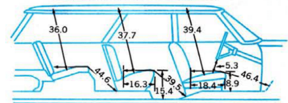
STATION WAGON DIMENSIONS*
