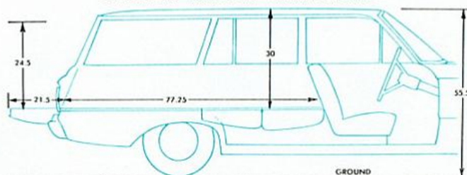
STATION WAGON DIMENSIONS
