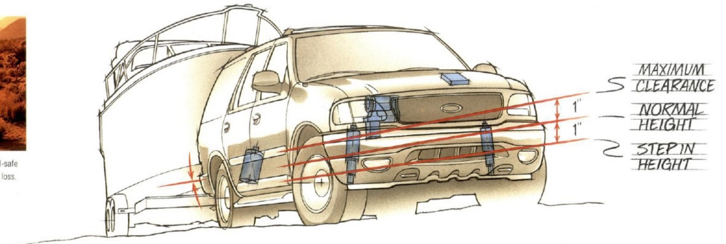
Expedition's technologically advanced load-leveling air suspension is designed to help improve ride and handling and trailer towing capability by keeping the vehicle at a constant normal height, while adjusting for changes in passenger, cargo and towing loads.
