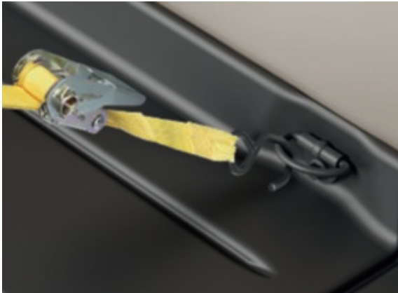
Integrated tie-downs points Transit Custom Van features side-mounted DIN/ISO compliant cargo tie-down points (standard).
