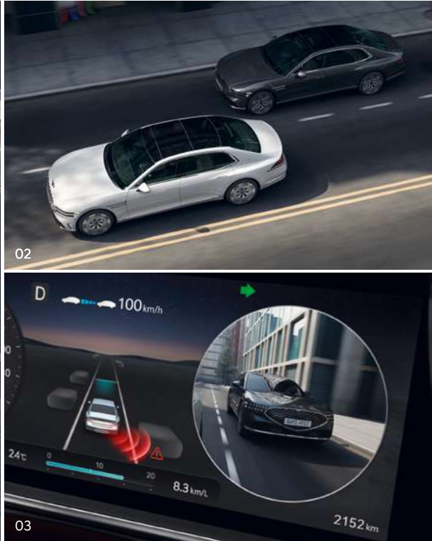
03. Blind-Spot View Monitor (BVM) system _ When the turn signals are activated, video images of the respective side/rear view of the vehicle appear on the center cluster.
