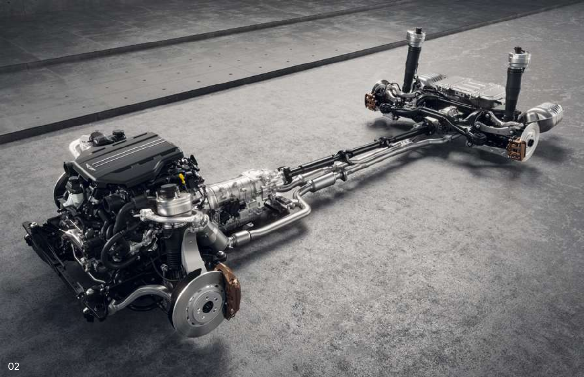
02. 3.5 turbo gasoline engine 48V electric supercharger _ An air-to-water intercooler system using an electric supercharger improves the vehicle's low and medium speed performance; its recharging capabilities via regenerative braking; and its responsiveness to torque assist, providing optimal performance.
