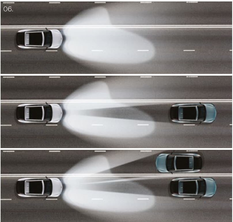
06. Intelligent Front-Lighting System (IFS) _ Allows the driver to use high beams at any time for optimized visibility by partially blocking the light in front of oncoming traffic or directly behind preceding vehicles to prevent glare for other drivers while still making it easier for you to drive at night.
