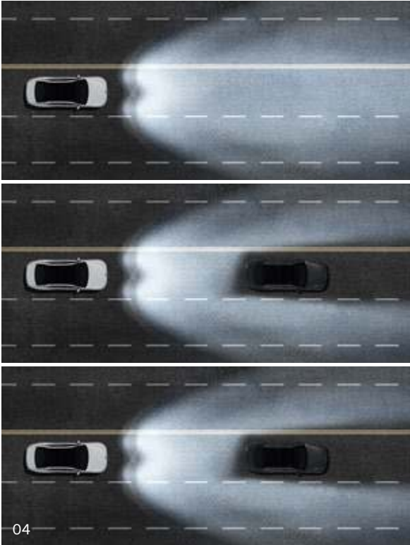
04. Intelligent Front-Lighting System (IFS) _ This keeps the high beam lights on constantly, automatically deactivating partially when an oncoming vehicle is detected, to prevent glare for the other driver. The same applies to vehicles in front. This makes driving at night easier as the high beam lights don't have to be adjusted manually.
