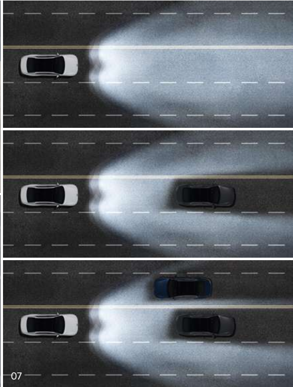
07. Intelligent Front-Lighting System (IFS) _ Situation-aware, always-on partial high beam dimming partially turns off the lights in the direction of oncoming traffic to prevent glare to drivers from the oncoming cars and ensures the visibility of the driver. The partial light control works the same for the preceding vehicles, and makes nighttime driving easier by eliminating the need to manipulate the headlamps separately.
