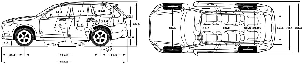
5-SEAT VERSION
