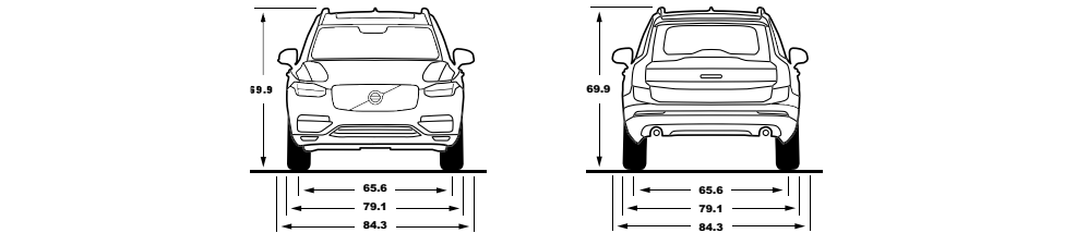
5-SEAT VERSION
