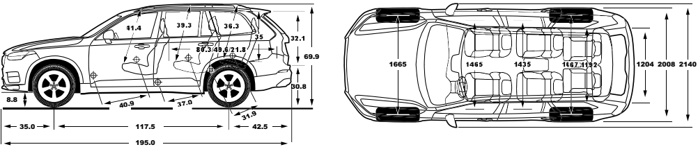
6-SEAT VERSION
