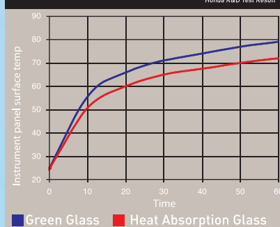
Heat Absorption Front Windshield helps keep the Interiors cool *Honda R&D Test Result
